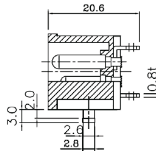
B-B SECTION
