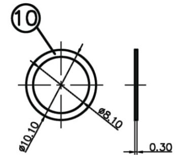
WASHER
