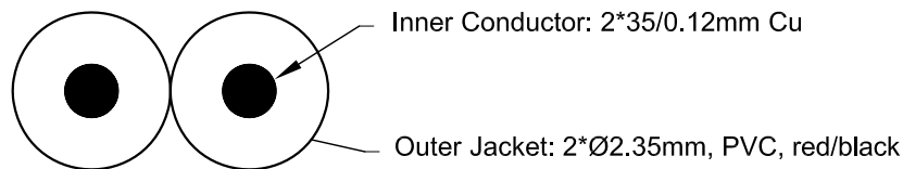
Cable Structure
