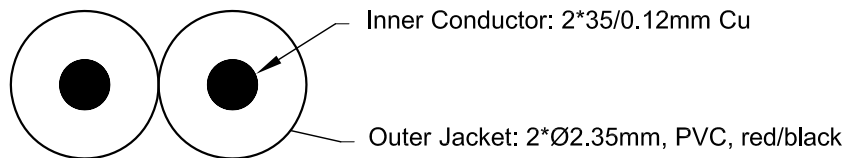
Cable Structure
