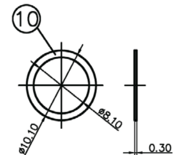
WASHER
