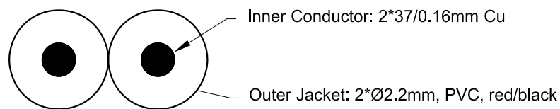
Cable Structure (0.75mm 2 )
