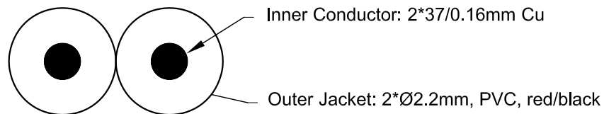
Cable Structure
