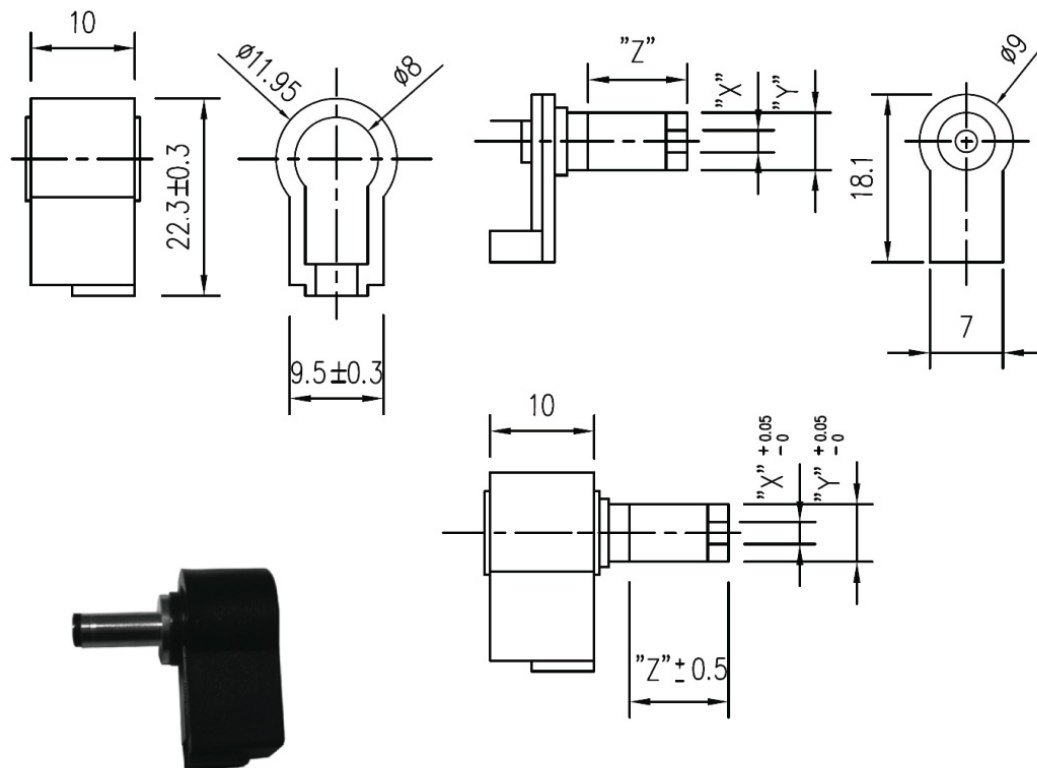
DC PLUG (RIGHT ANGLE TYPE)
