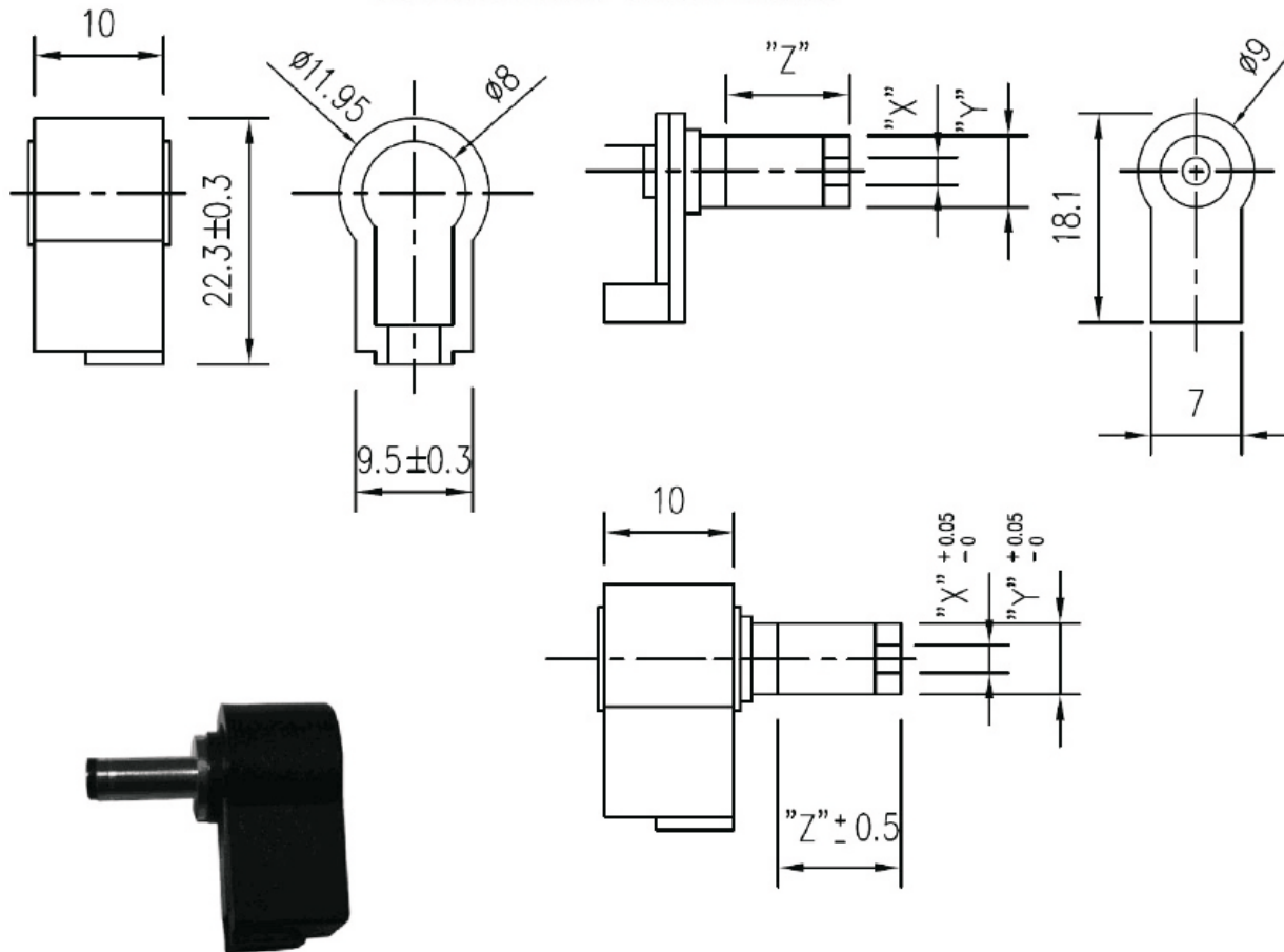
DC PLUG (RIGHT ANGLE TYPE)
