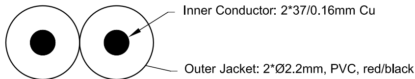
Cable Structure
